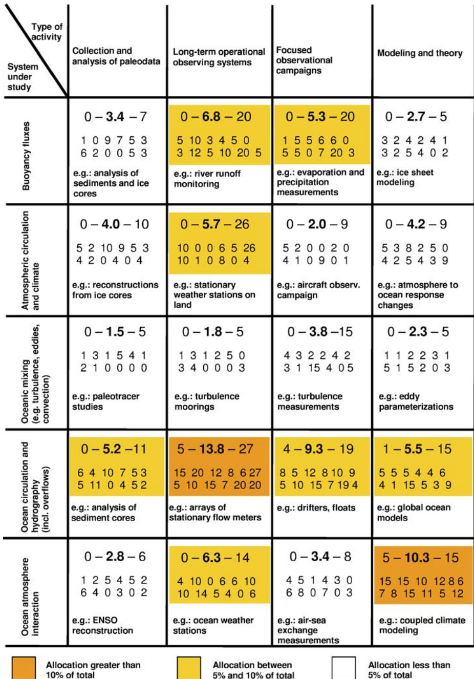
Fig. 9 Experts' judgments concerning the allocation of a research budget of 500-million US dollars per year across the 20 areas of climate research. Results are given in percentage of the total budget
