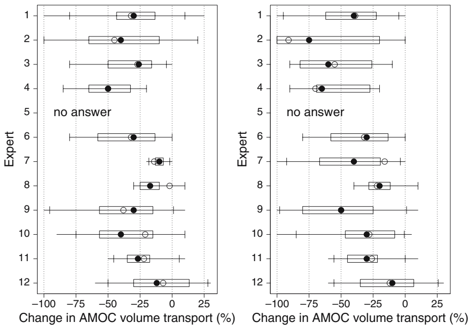
Fig. 3 Change in AMOC strength in the year 2100 in percent of the present-day value for a doubling (left panel) and quadrupling (right panel) of the pre-industrial CO 2 concentration. Shown are the complete ranges (horizontal lines), the 90%-quantiles (vertical tick marks), the 50%-quantiles (boxes) and the medians (solid dots) from experts' elicited probability distributions. The experts' best estimates (open dots) are derived from Fig. 2
