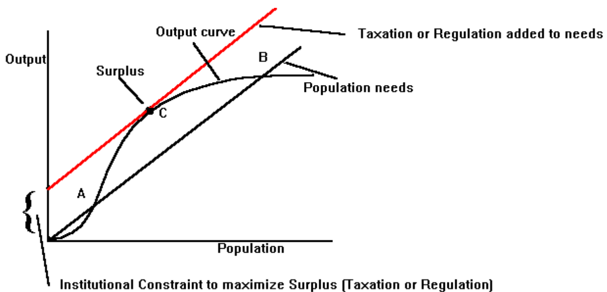
Figure 1: The Malthusian Model
