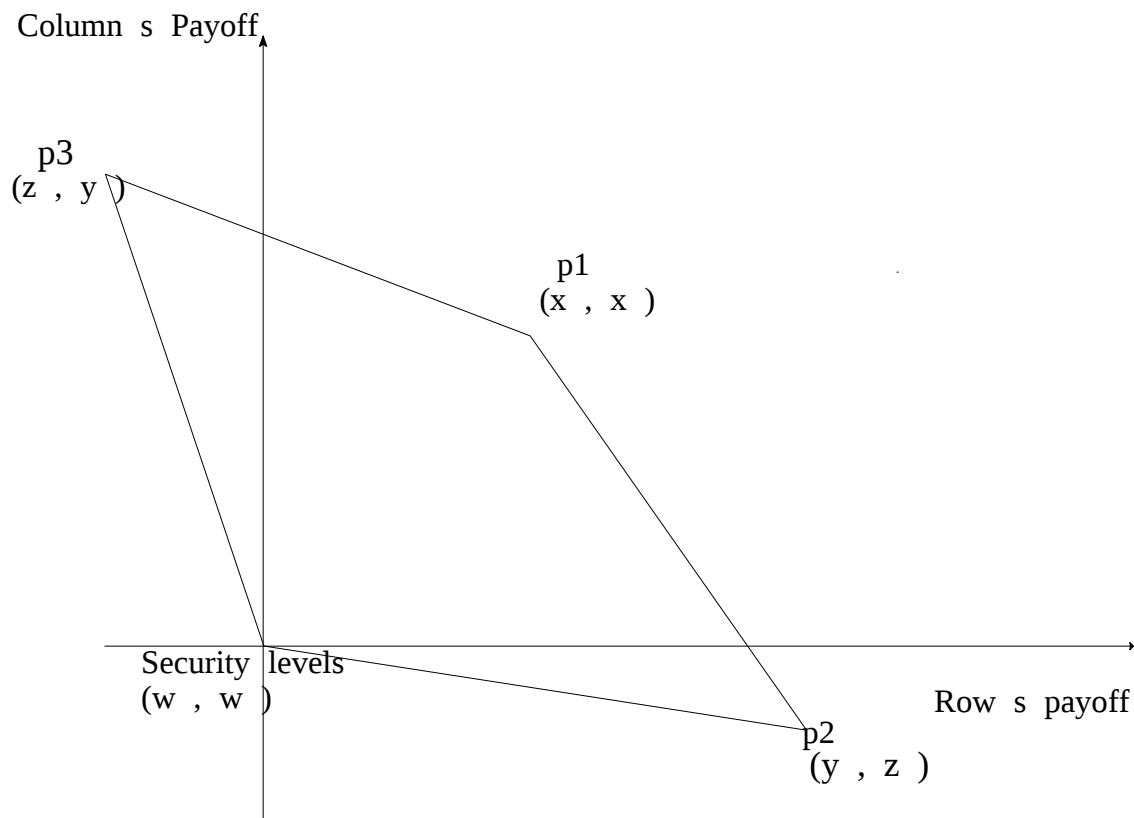
Figure 3: Feasible Average Payoffs
